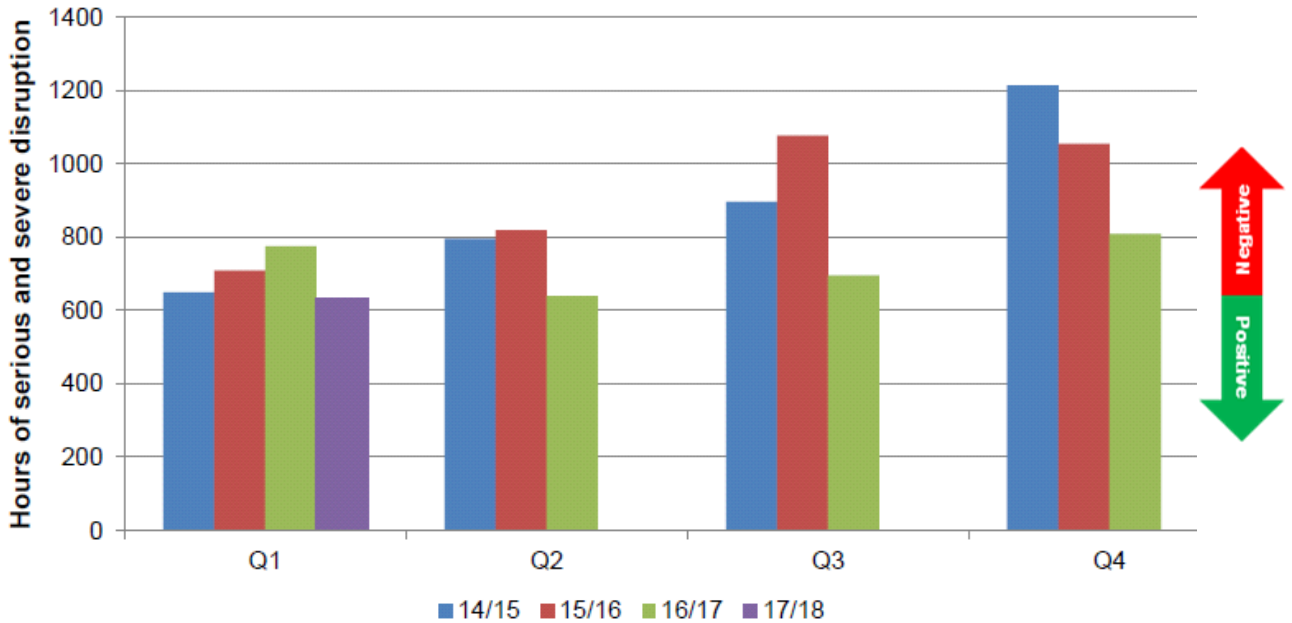
Graph 3 - Duration of TLRN serious & severe unplanned and planned events (hrs) by financial quarters, Q1 2014-15 to Q1 2017-18
