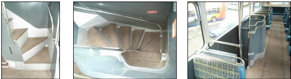
Fig 2 : DMS staircase
